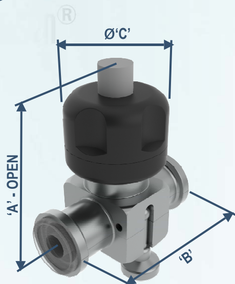
Manual Valve:
